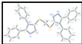
Fig. 1. View of (I) showing the atom-labelling scheme [symmetry code: (A) -x + 1, y, -z + 1/2 ]. Displacement ellipsoids are drawn at the 50% probability level.
